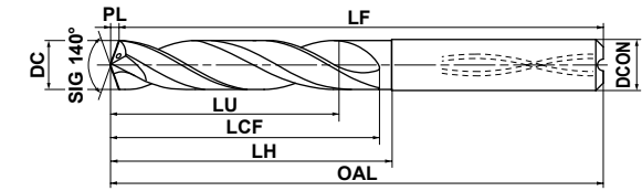
● Type 2 Cylindrical shank type
