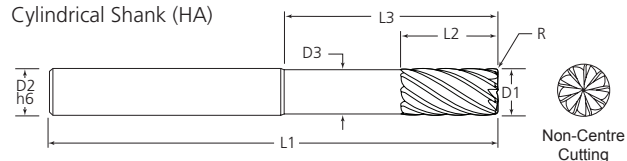
Cylindrical Shank (HA)
